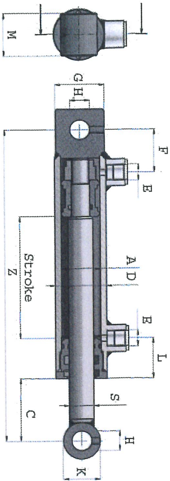
HYDRAULICS CYLINDERS SERIES CVDV
